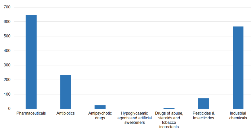
Figure 26: Cumulated PNEC exceedance of organic chemicals for chemical groups
