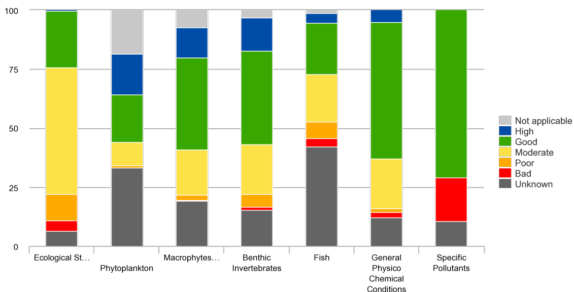
Figure 66: Ecological status: classification of biological quality elements and physico-chemical conditions (indicated as % of the total length) 73
