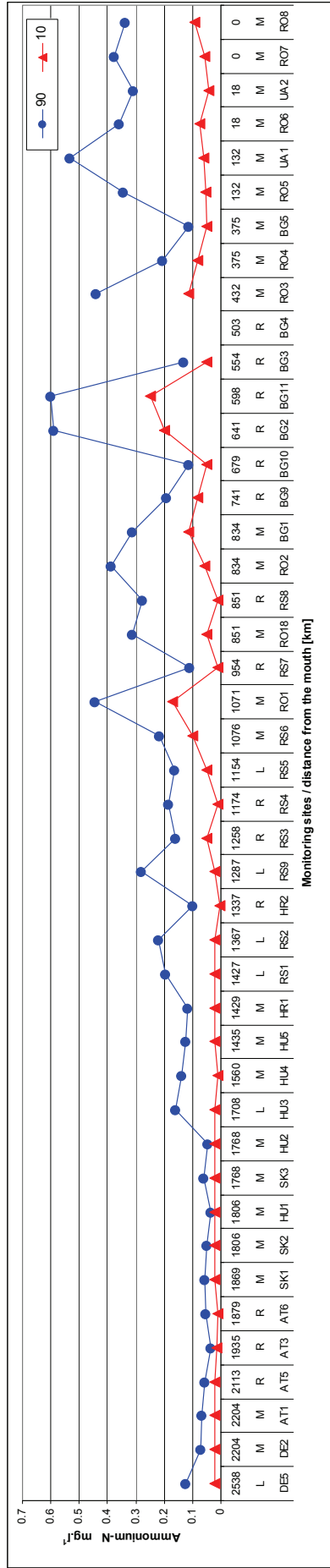
Figure 4.26: The percentile (90, 10) of N-NH 4 concentration along the Danube river in 2007.
