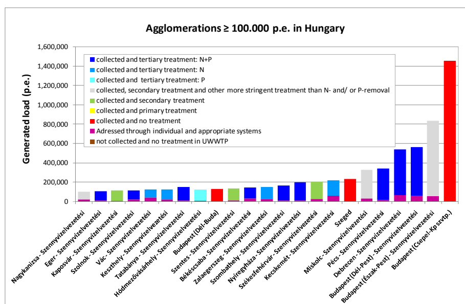
Figure 15: Wastewater treatment in agglomerations \geq 100,000 PE in the Hungarian part of the DRB
